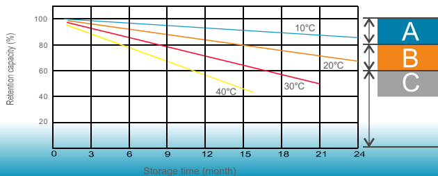
Self Discharge Characteristics
